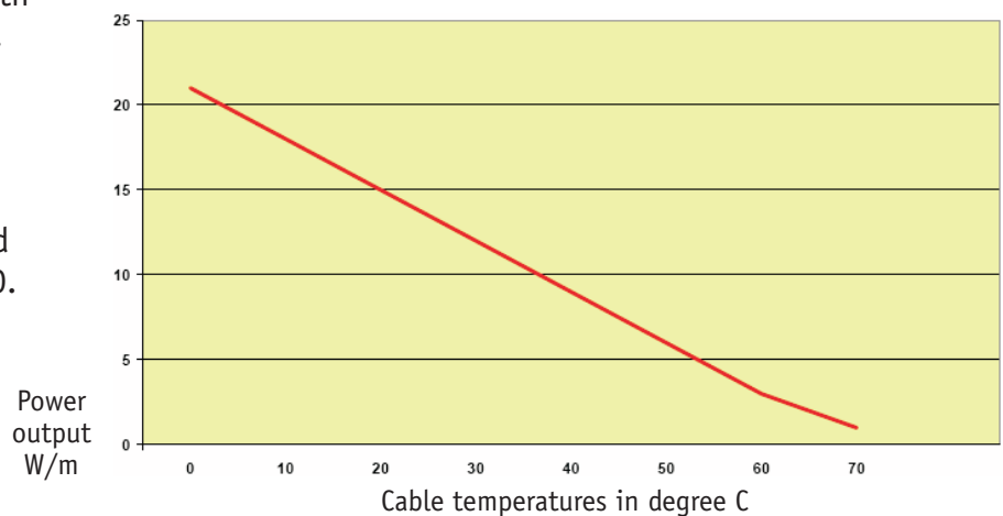
Nominell poweroutput K3 at different cable temperatures.
